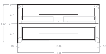
1200mm Front View
