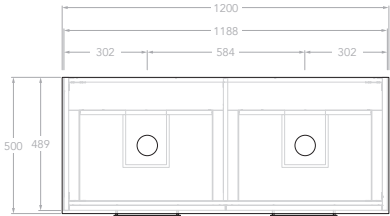
Top View Double
