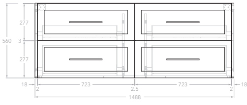
1500mm Front View
