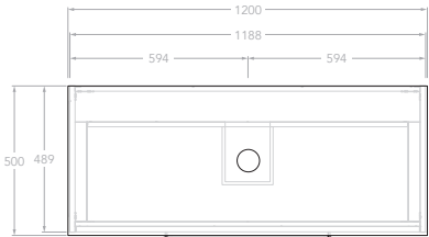
Top View Centre
