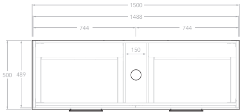
Top View Double
