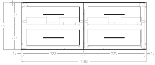
1500mm Front View
